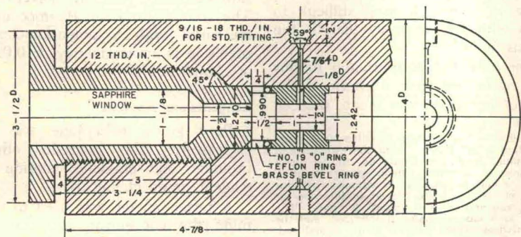
Fig. 2. High-pressure cell.
