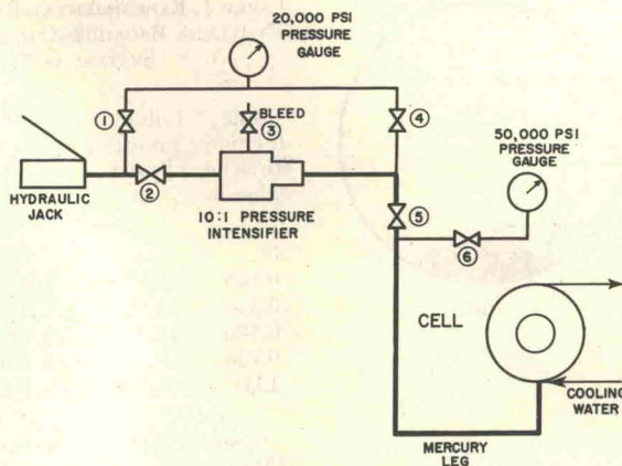
Fig. 3. Experimental apparatus.
